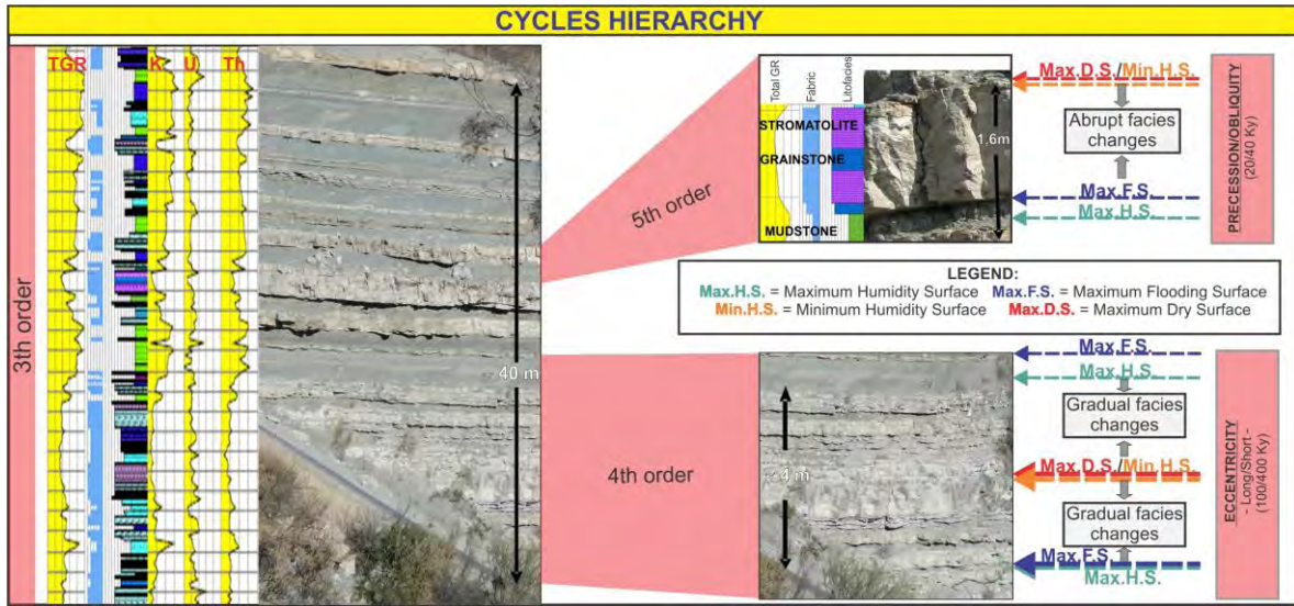
Figure 1 - 3 rd , 4 th and 5 th order cycles in Balbuena Sequence 4, Cabra Corral Dam area.
