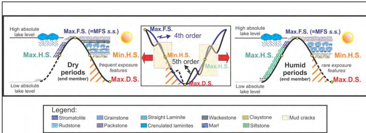
Figure 2 – High resolution environmental conditions and facies distribution of 4 th (central square) and 5 th orders cycles in Balbuena Sequence 4 (3 rd order dry periods to the left and humid periods to the right), Cabra Corral Dam area. Max.H.S.= Maximum Humid Surface; Min.H.S.= Minimum Humid Surface; Max.F.S.=Maximum Flooding Surface; Max.D.S.=Maximum Dry Surface.
